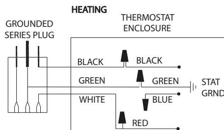
Figure 5. TF115P-002. Wiring for HEATING
