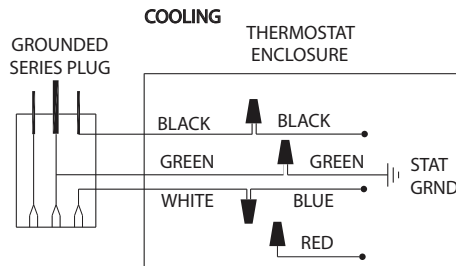
Figure 3. TF115P-002. Wiring for COOLING.
